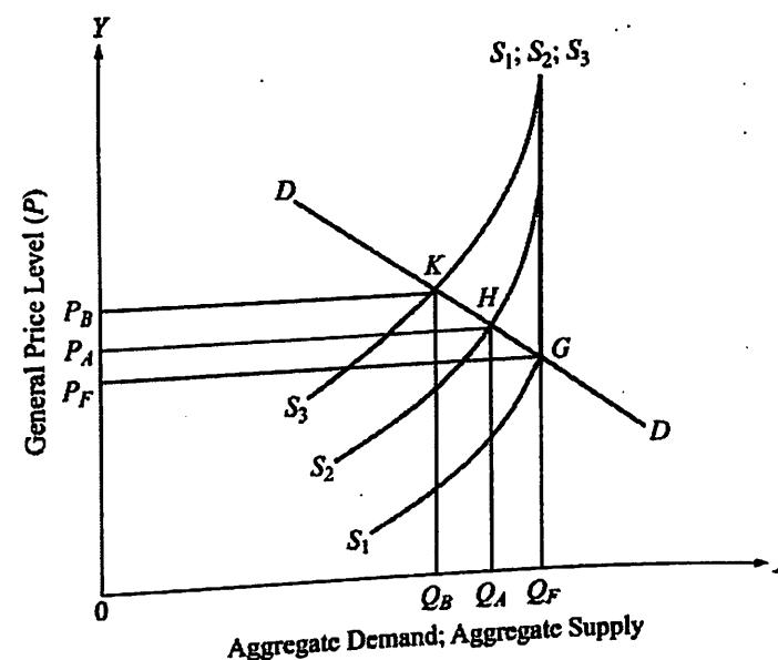
Fig. 7.3 Cost-push Inflation
