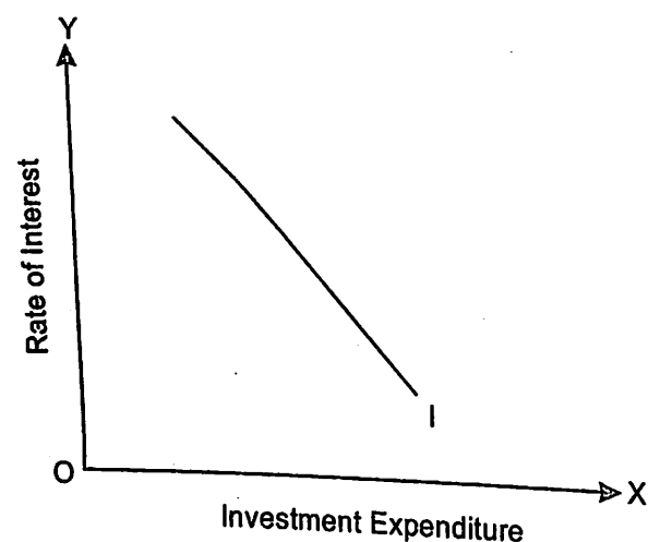
Fig. 2.6 Investment Curve
