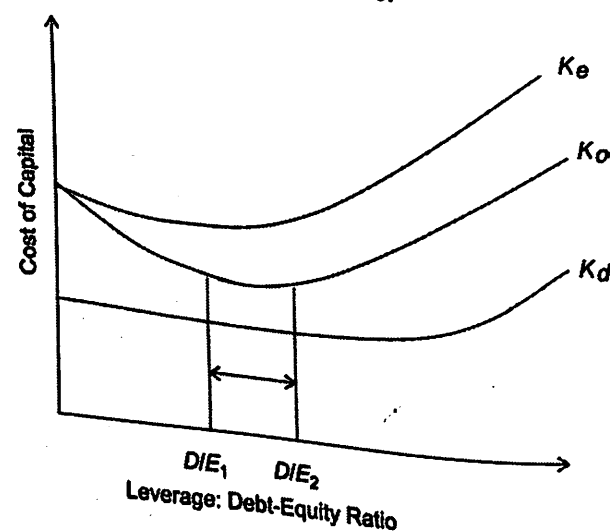
Fig. 8.9 Traditional Approach
