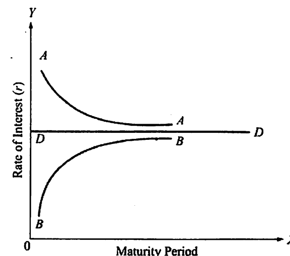
Fig. 1.7 IS Curve
